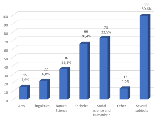
Fig. 1.5 Main subjects/fields of teaching (N=324)
